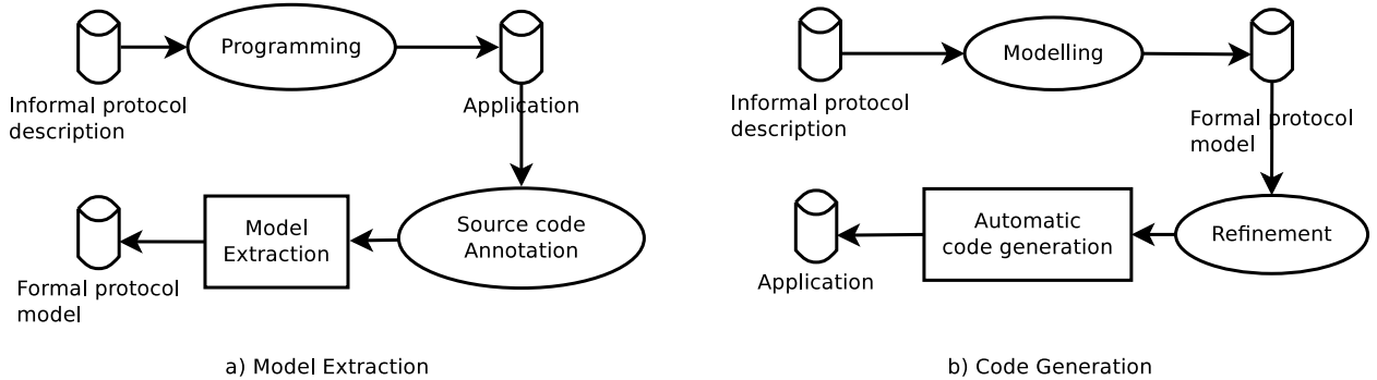
Fig. 1. Typical workflows used by a) model extraction; b) code generation.
